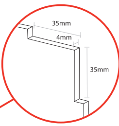
Corner detail (all 4 corners)
